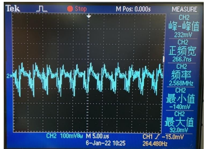
Output ripple (5V / 6A)
