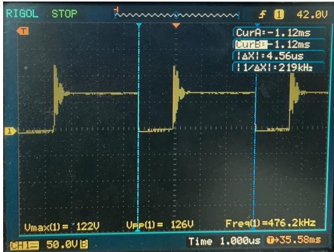
Transformer Switch Waveform
