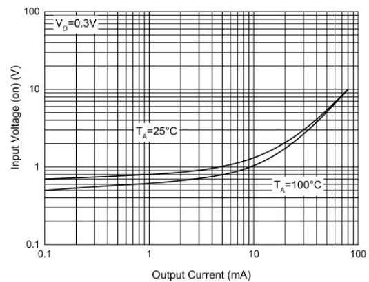
DTR1 Input Voltage (on) Characteristics
