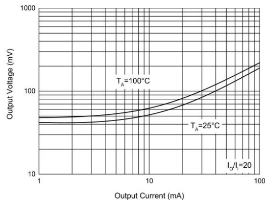
DTR1 Output Voltage Characteristics
