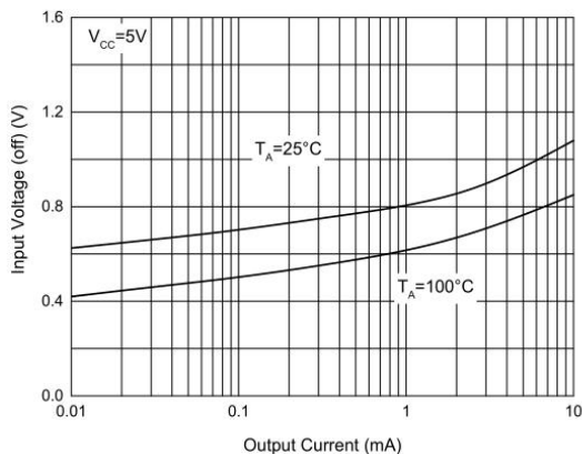
DTR1 Input Voltage (off) Characteristics
