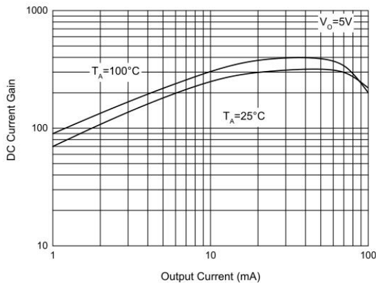
DTR1 DC Current Gain Characteristics
