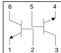
Equivalent Circuit
