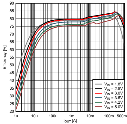
图 9-2. Efficiency at 0.4 V_{OUT}
