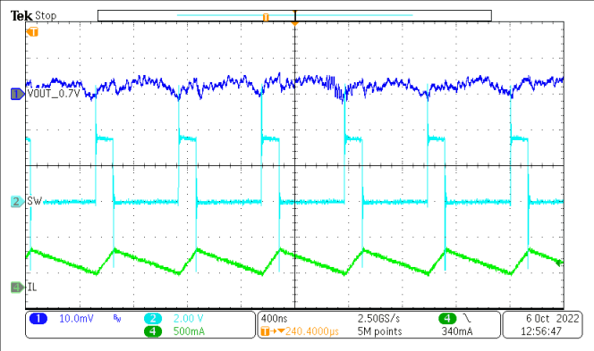
图 9-15. Typical Operation at 0.7 V OUT , 400 mA I OUT
