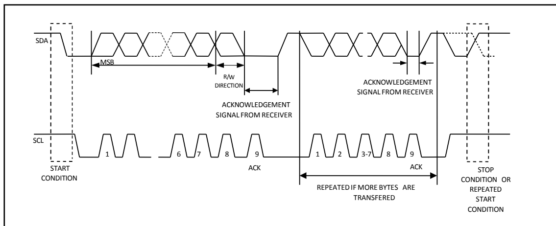
Figure 6-2. Data Transfer on I2C Serial Bus
