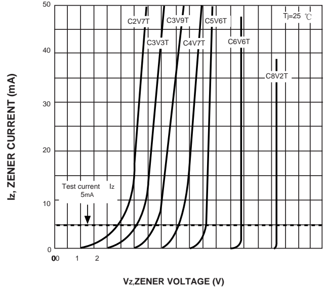
FIG. 2-ZENER BREAKDOWN CHARACTERISTICS
