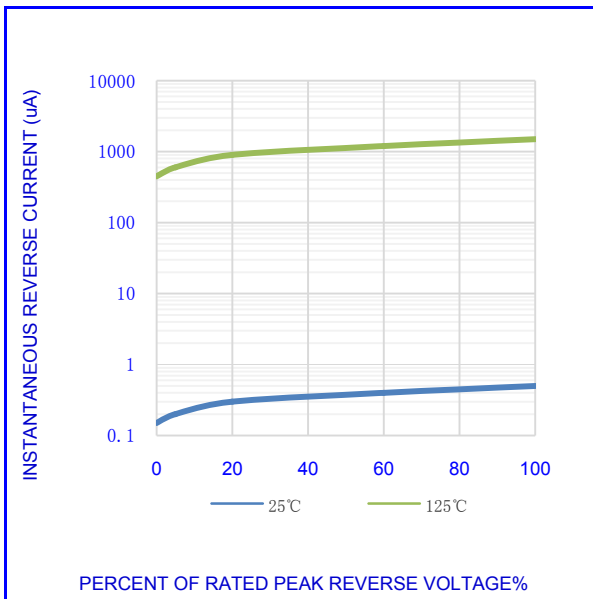
Fig.3-TYPICAL REVERSE CHARACTERISTICS
