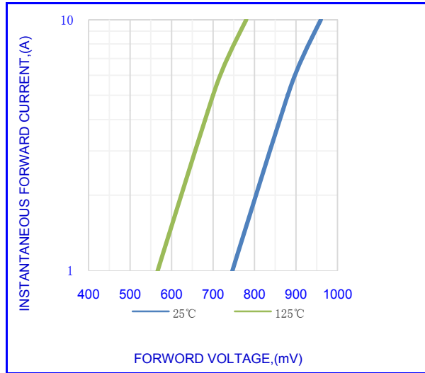
Fig.2-TYPICAL INSTANTANEOUS FORWARD
