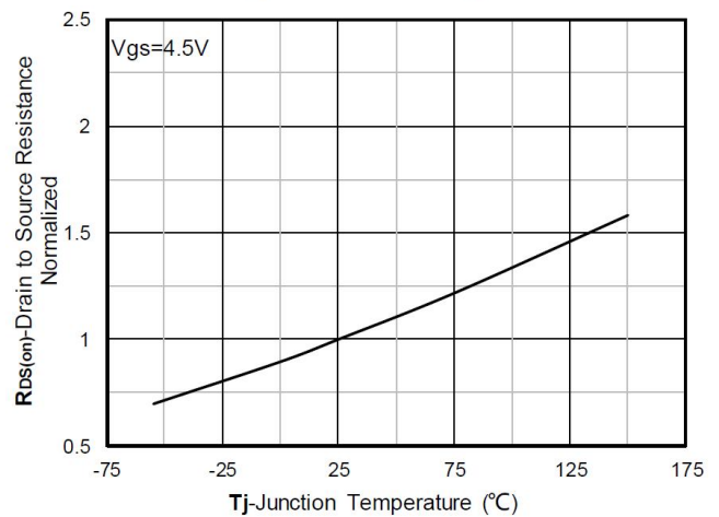
Figure6. Normalized On-Resistance
