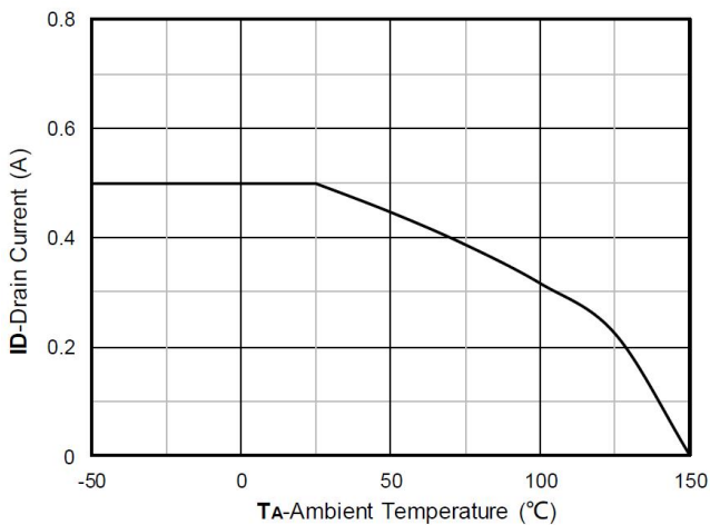
Figure11. Current dissipation
