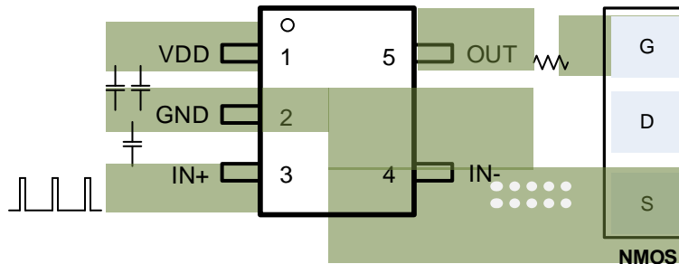
Figure 16. 1EDN7512 PCB Layout Example
