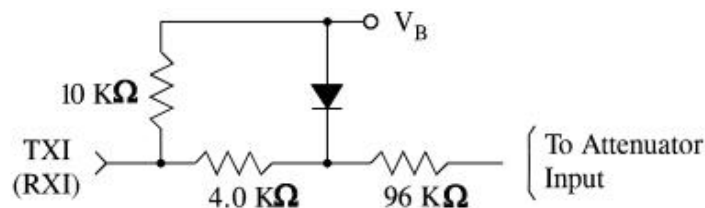
Figure 1. Attenuator Input Stage
