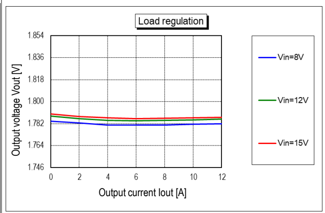
Vout vs. Line Voltage and Load Current @ +25degC. (Vout = 1.8V)
