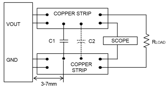
C1=220uF x 3 CERAMIC C2=OPEN
