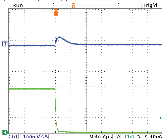
Step Load Transient Response (Vin=12V, Vout=5V, Load=10x10µF X5R 0805 ceramic, plus 1x470µF, 7mΩ POSCAP, total 570µF, Iout=3A to 0A) Top trace=Vout, Bottom trace=Iout
