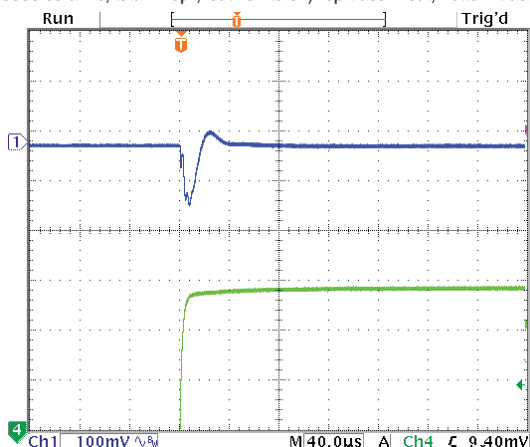
Step Load Transient Response (Vin=12V, Vout=5V, Cload=12x10μF X5R 0805 ceramic, total 120μF, Iout=0A to 3A) Top trace=Vout, Bottom trace=Iout
