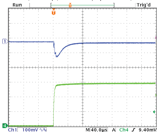
Step Load Transient Response (Vin=7.5V, Vout=5V, Load=10x10µF X5R 0805 ceramic, plus 1x470µF, 7mΩ POSCAP, total 570µF, Iout=0A to 3A) Top trace=Vout, Bottom trace=Iout
