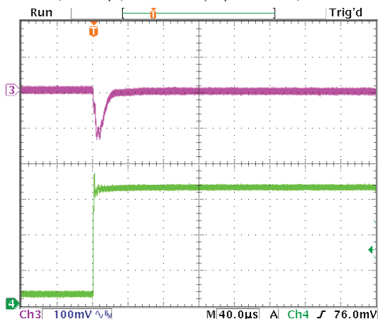
Step Load Transient Response (Vin=7.5V, Vout=5V, Cload=5x10μF X5R 0805 ceramic, total 50μF, Iout=0A to 3A) Top trace=Vout, Bottom trace=Iout
