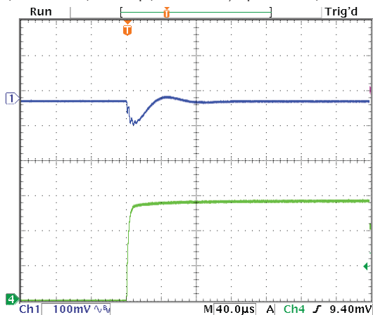
Step Load Transient Response (Vin=12V, Vout=5V, Load=10x10µF X5R 0805 ceramic, plus 1x470µF, 7mΩ POSCAP, total 570µF, Iout=0A to 3A) Top trace=Vout, Bottom trace=Iout
