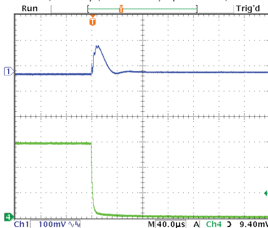
Step Load Transient Response (Vin=7.5V, Vout=5V, Load=10x10µF X5R 0805 ceramic, plus 1x470µF, 7mΩ POSCAP, total 570µF, Iout=3A to 0A) Top trace=Vout, Bottom trace=Iout
