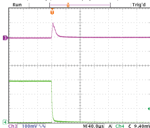
Step Load Transient Response (Vin=12V, Vout=5V, Cload=12x10μF X5R 0805 ceramic, total 120μF, Iout=3A to 0A) Top trace=Vout, Bottom trace=Iout
