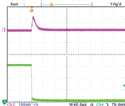
Step Load Transient Response (Vin=7.5V, Vout=5V, Cload=5x10μF X5R 0805 ceramic, total 50μF, Iout=3A to 0A) Top trace=Vout, Bottom trace=Iout
