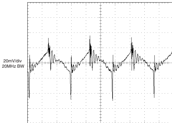
UWR-3.3/9-D24A Output Ripple and Noise (PARD) (V IN = 24V, full load, external 0.47μF output capacitor.)
