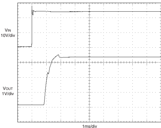
UWR-3.3/9-D48A Start-Up from V IN (V IN = 48V, full load, external 0.47μF output capacitor.)
