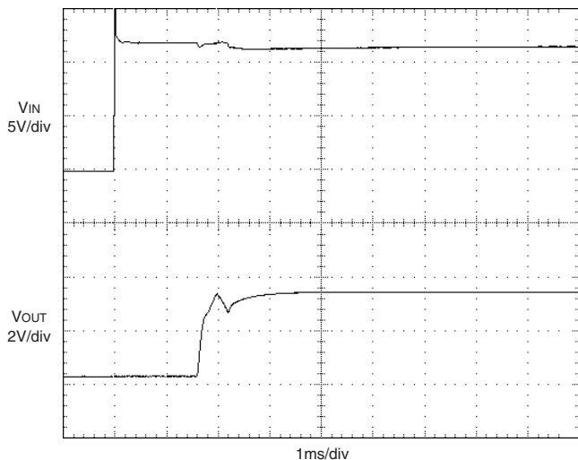
UWR-3.3/9-D24A Start-Up from V IN (V IN = 24V, full load, external 0.47μF output capacitor.)
