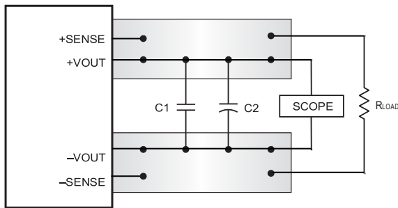
C1 = 1μF C2 = 10μF LOAD 2-3 INCHES (51-76mm) FROM MODULE Figure 3. Measuring Output Ripple/Noise (PARD)
