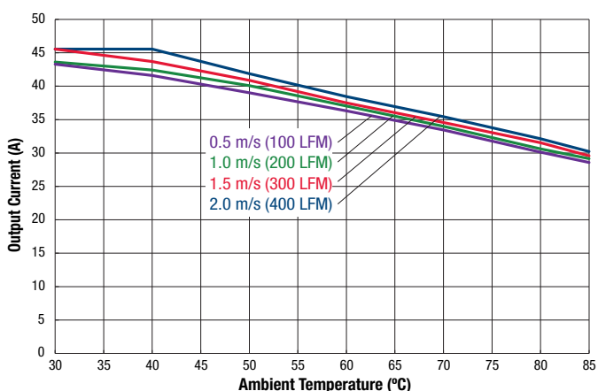
Maximum Current Temperature Derating at Sea Level (Vin = 75V, without baseplate. Airflow Direction Is Longitudinal from Vin to Vout.)
