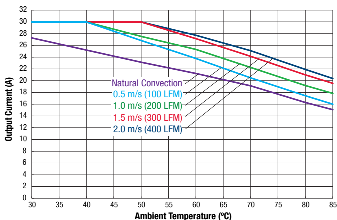
Maximum Current Temperature Derating at Sea Level (Vin = 36V, no baseplate. Airflow Direction Is Longitudinal from -Vin to +Vin.)
