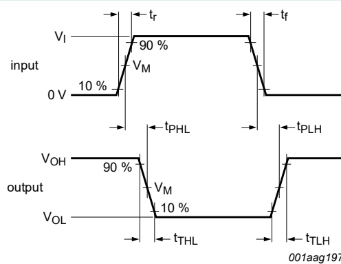
Fig. 4. Propagation delay, output transition time
