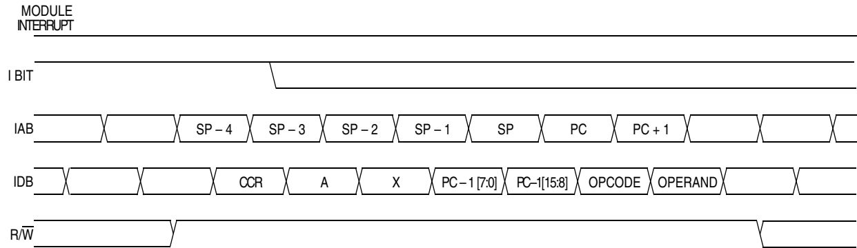
Figure 7-9. Interrupt Recovery
