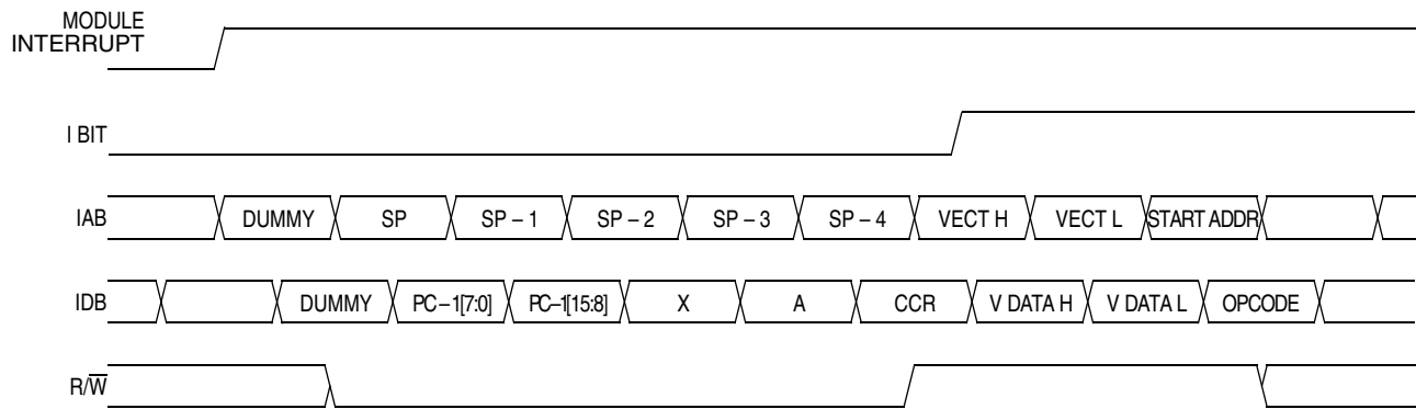
Figure 7-8. Interrupt Entry
