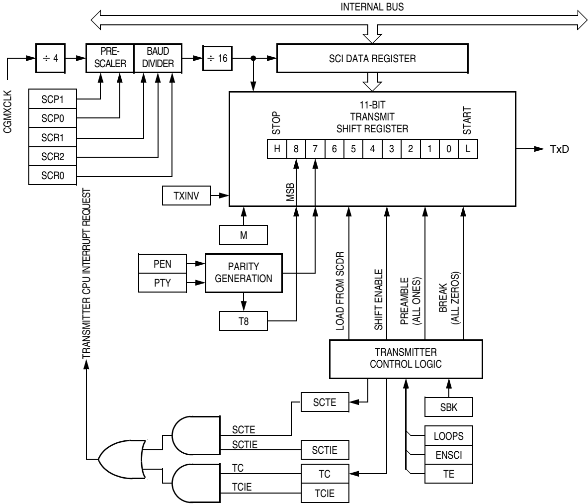
Figure 16-4. SCI Transmitter
