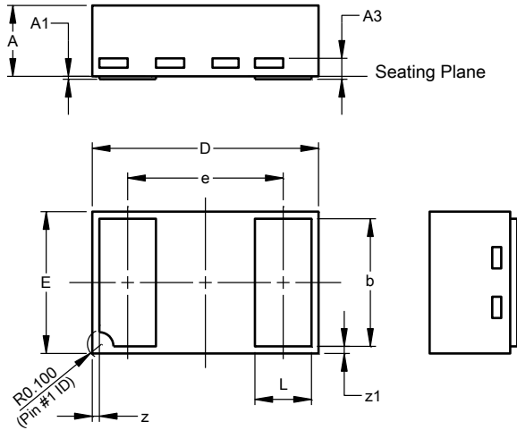
U-DFN1610-2 (Type B)
