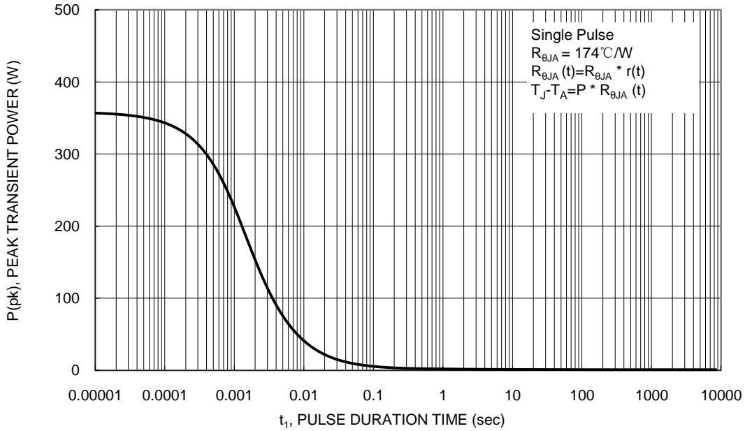
Figure 13. Single Pulse Maximum Power Dissipation
