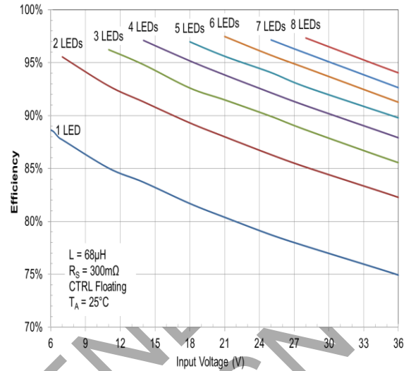
Figure 14 Efficiency vs. Input Voltage
