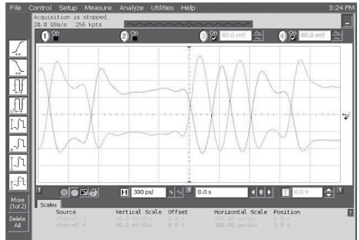
Data Waveforms, 3.0Gbps (left) & 6.0Gbps (right)
