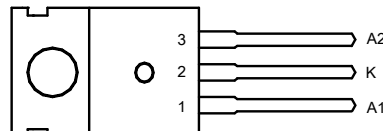
TO-220-3 (2)
