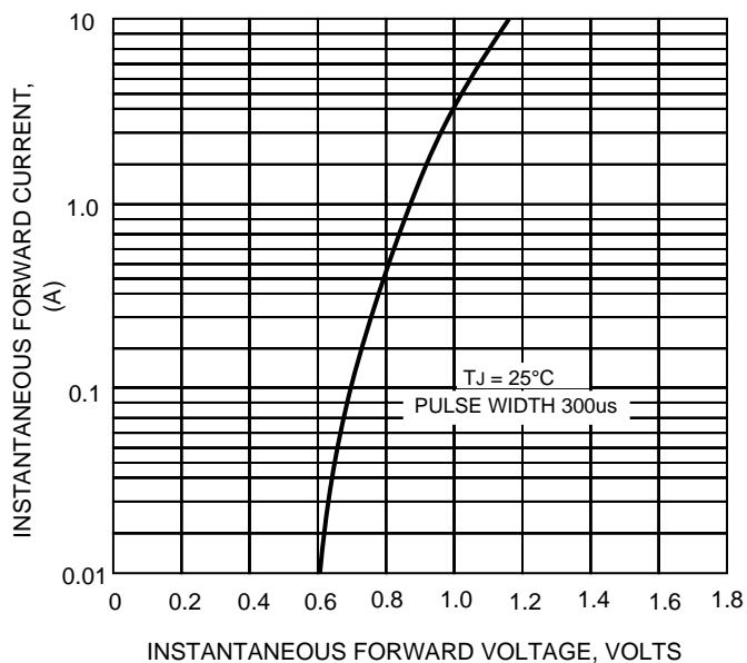
FIG.4-TYPICAL FORWARD CHARACTERISTICS
