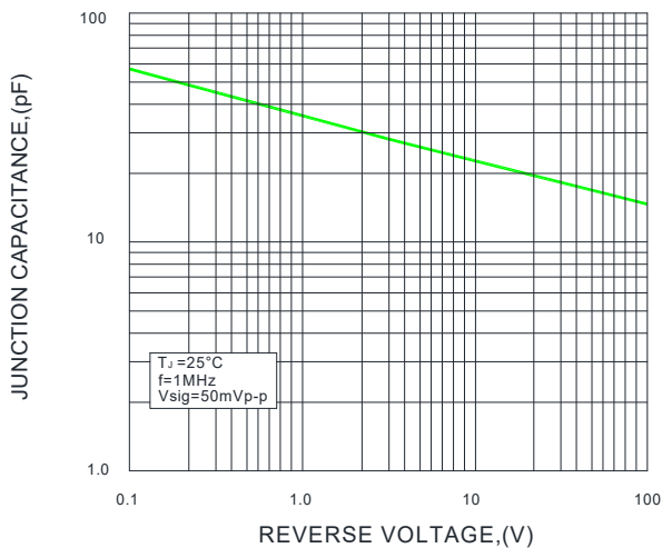
FIG.5-TYPICAL JUNCTION CAPACITANCE
