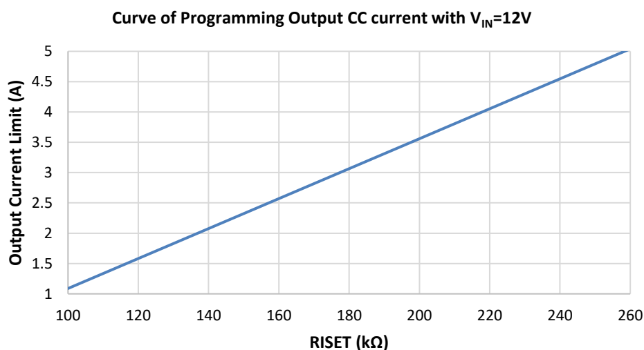
Figure 4. Curve of Programming Output CC Current
