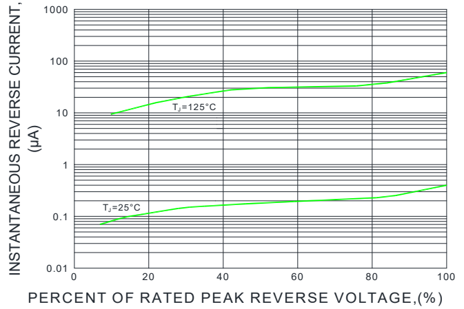
FIG.4-TYPICAL REVERSE CHARACTERISTICS
