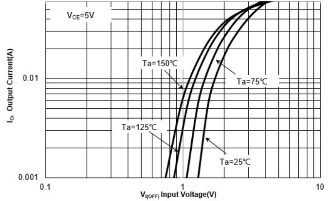
Fig 2. Collector Current vs. V_{I(OFF)}
