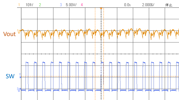
Switching Waveform at I_{out} = 1\text{A} ( V_{in} = 12\text{V} , V_{out} = 3.3\text{V} )
