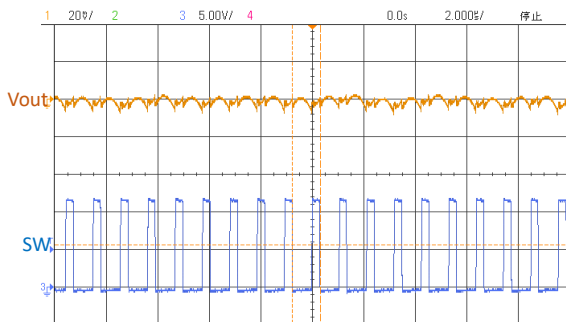
Switching Waveform at I_{out} = 0\text{A} ( V_{in} = 12\text{V} , V_{out} = 3.3\text{V} )
