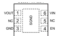
DFN2x2-6L
