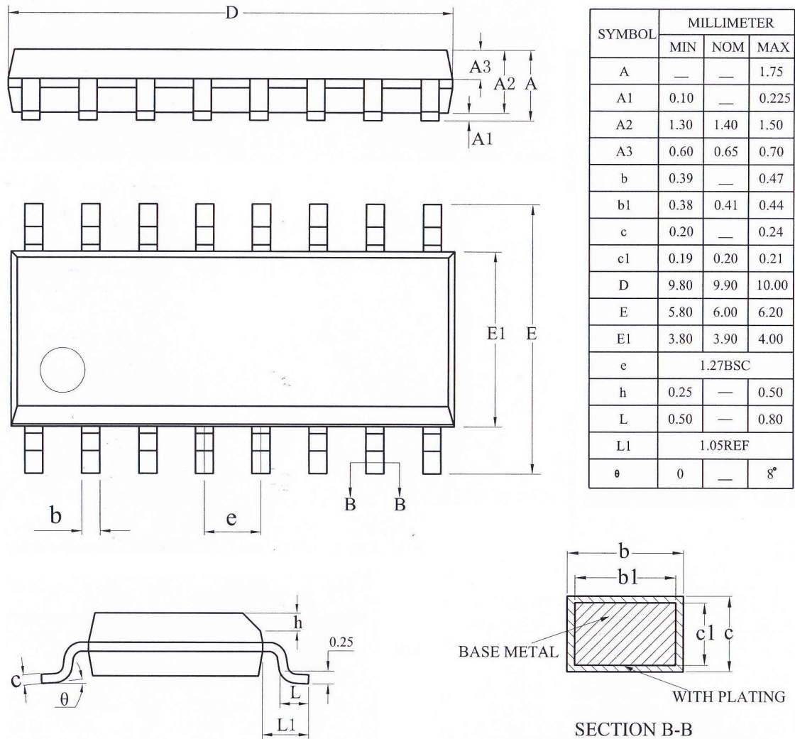
Figure 3-1. AD142A4_SOP16 Package
