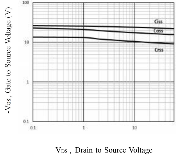
Fig.4 Capacitance Characteristics
