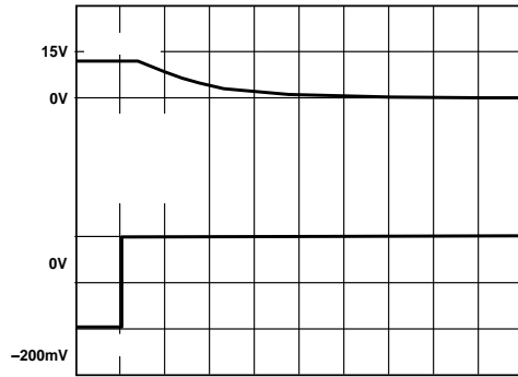
TIME (4µs/DIV) Figure 19. Negative Overtolerance Recovery
