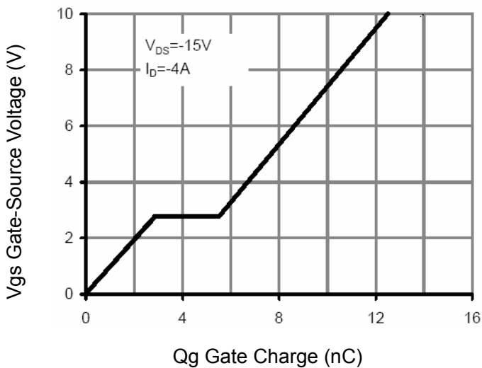
Qg Gate Charge (nC) Figure 11 Gate Charge
