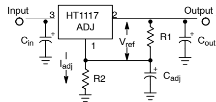
Figure 24. Adjustable Output Regulator
