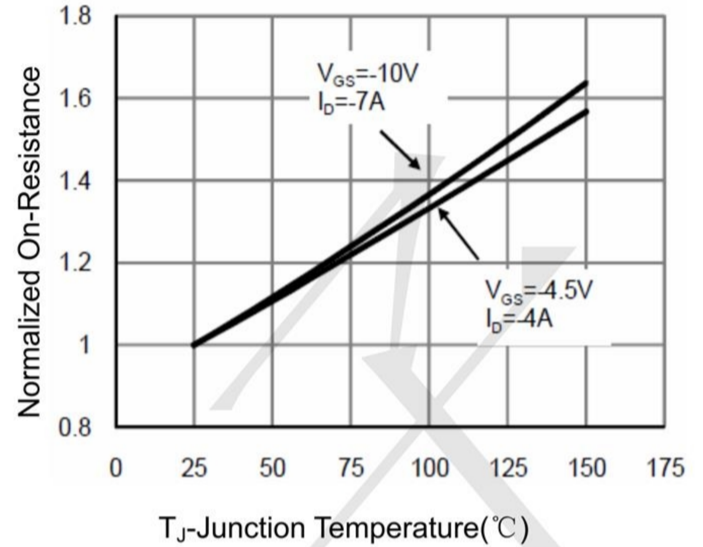
Figure 4 Rdson-Junction Temperature
