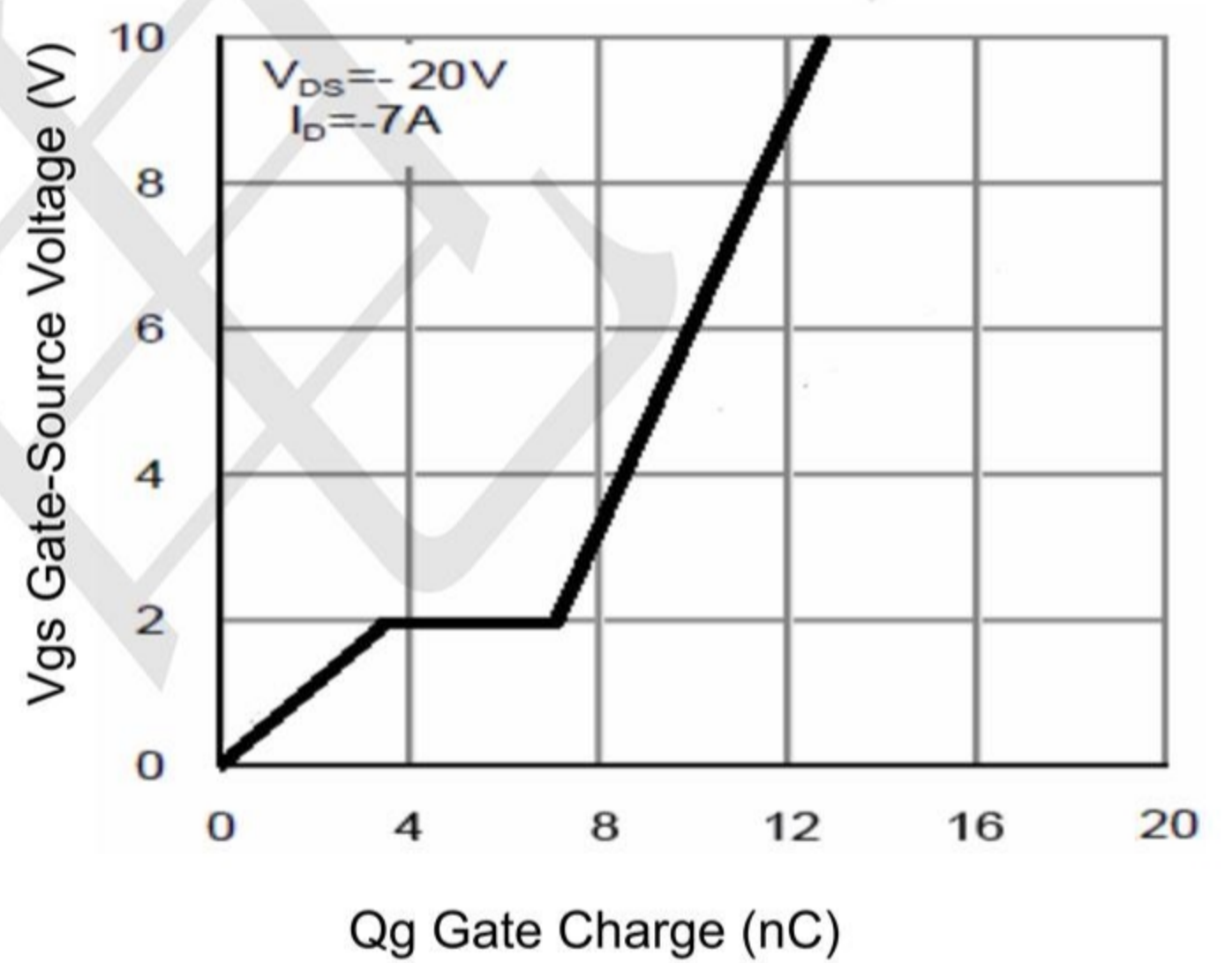
Figure 5 Gate Charge
