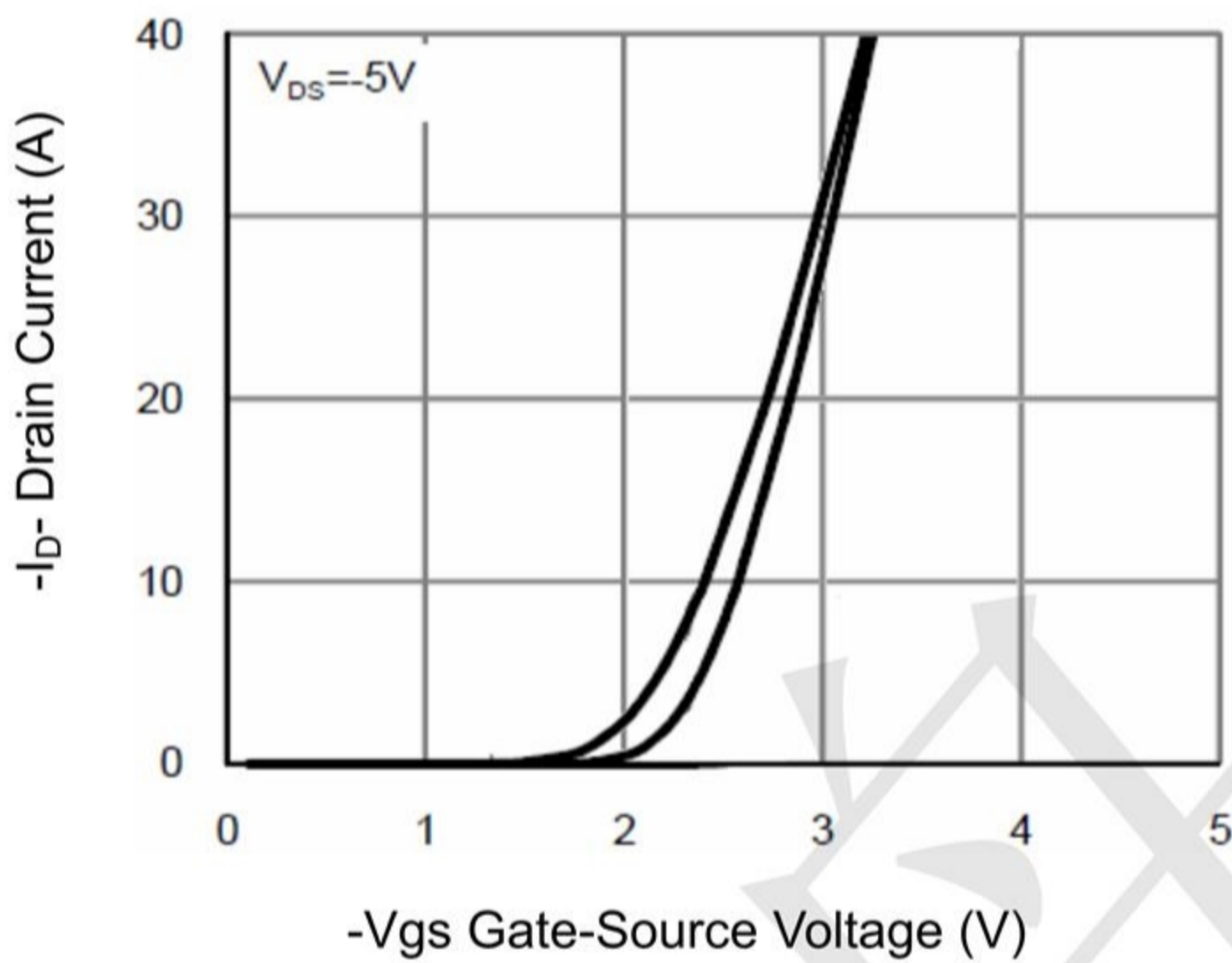
Figure 2 Transfer Characteristics
