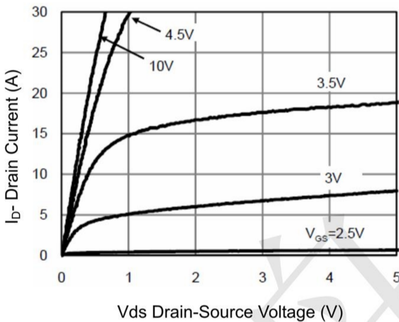
Figure 3 Output Characteristics
