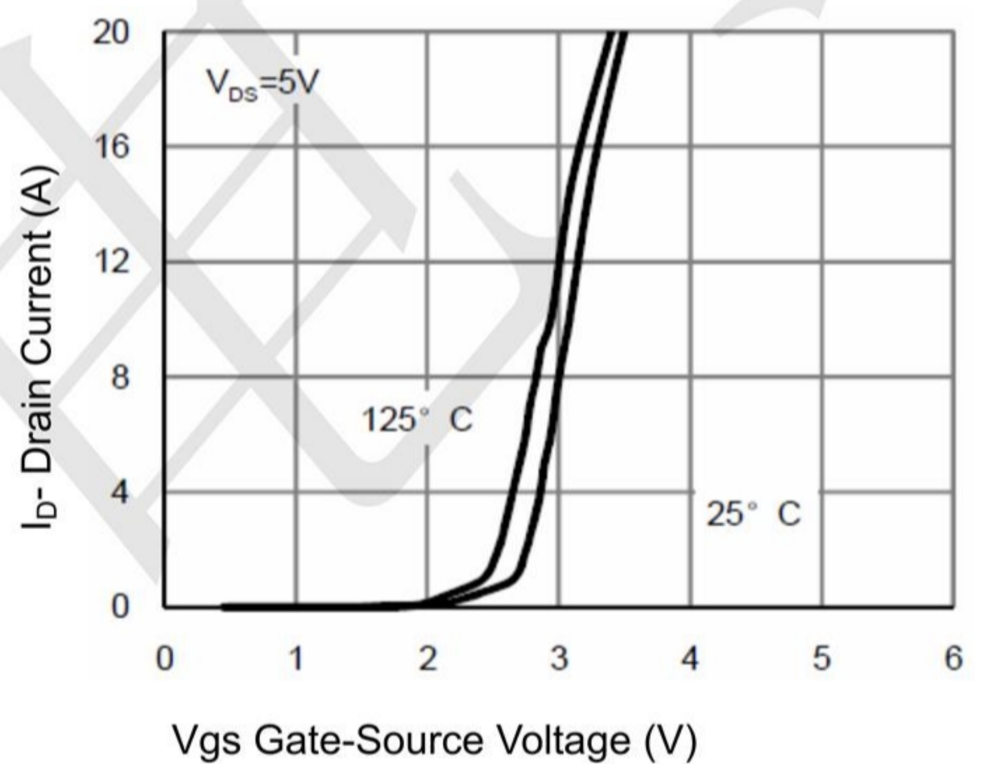
Figure 4 Transfer Characteristics
