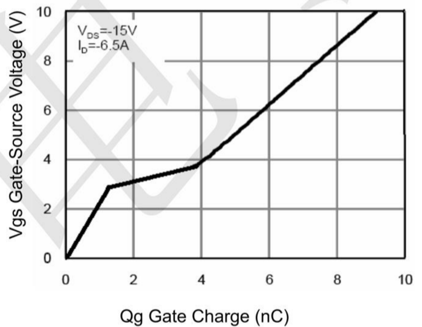
Figure 5 Gate Charge
