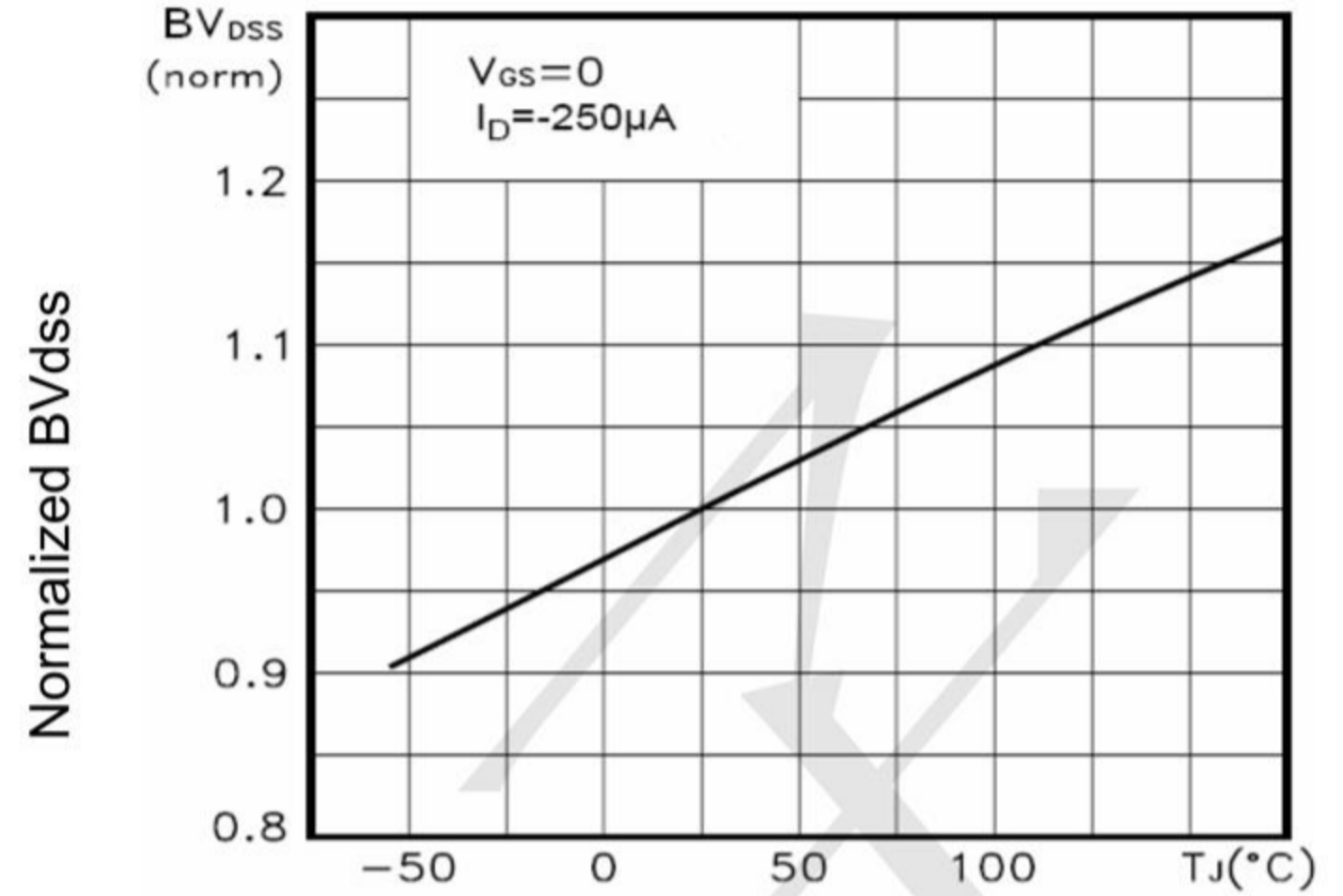
Figure 9 BV DSS vs Junction Temperature
