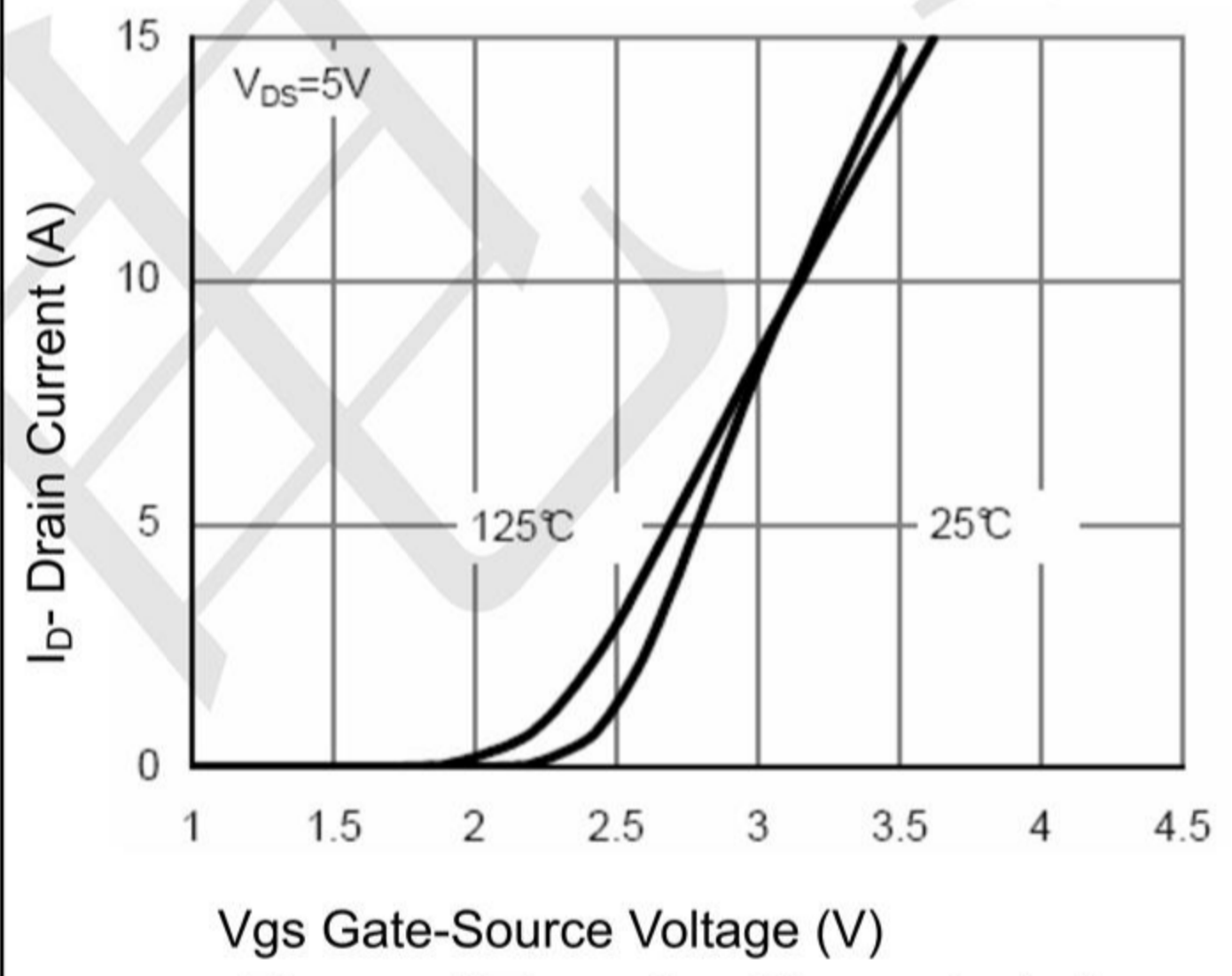
Figure 4 Transfer Characteristics
