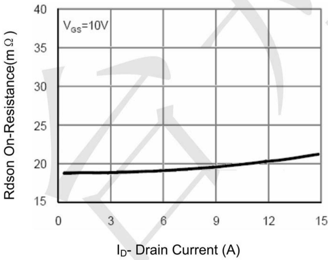
Figure 5 Drain-Source On-Resistance
