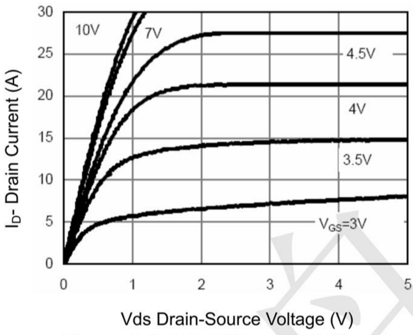
Figure 3 Output Characteristics
