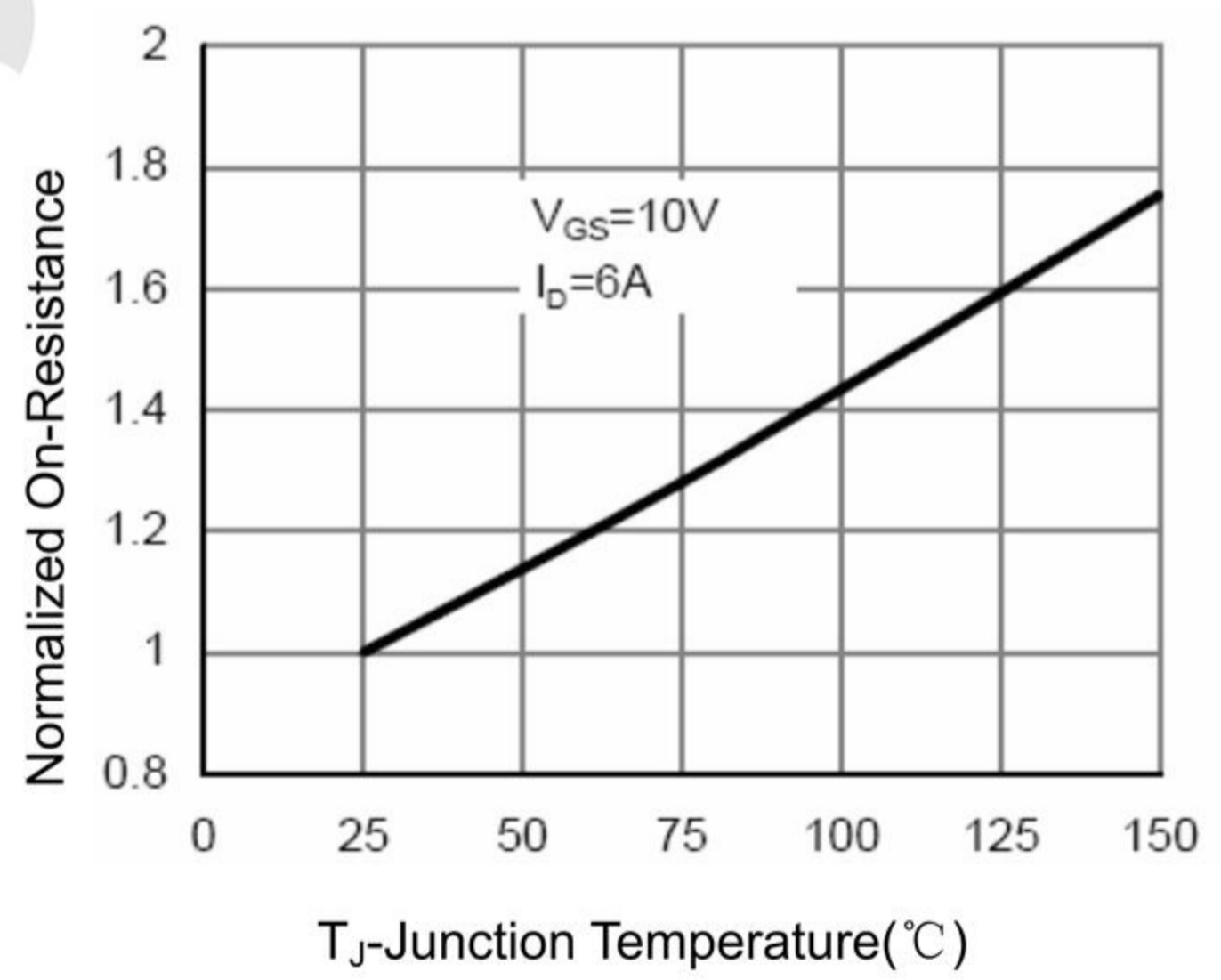
Figure 6 Drain-Source On-Resistance
