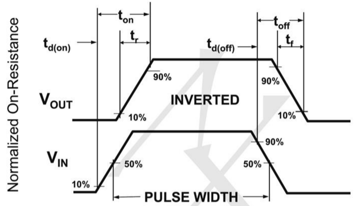
Figure 2: Switching Waveforms
