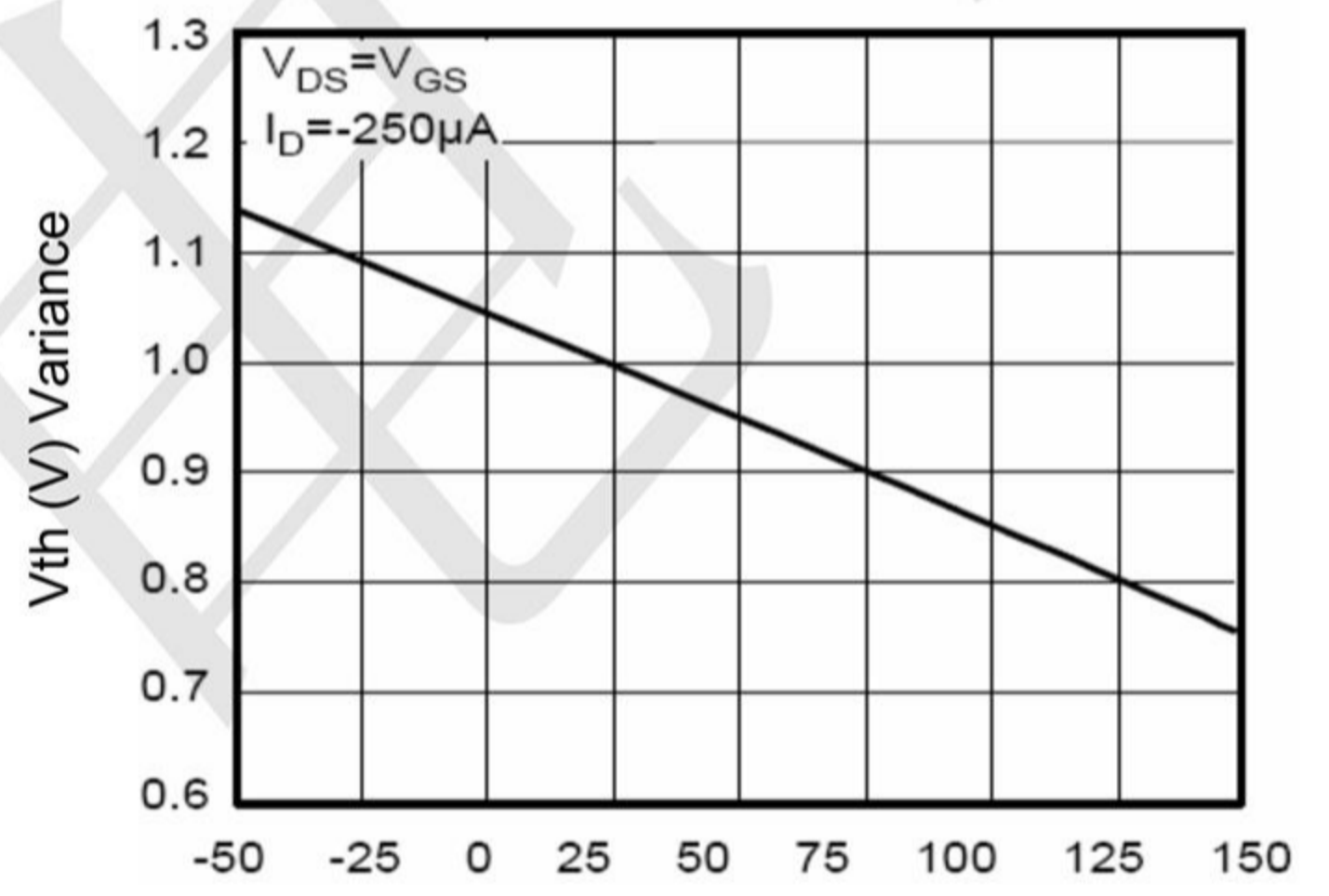
Figure 10 V GS(th) vs Junction Temperature
