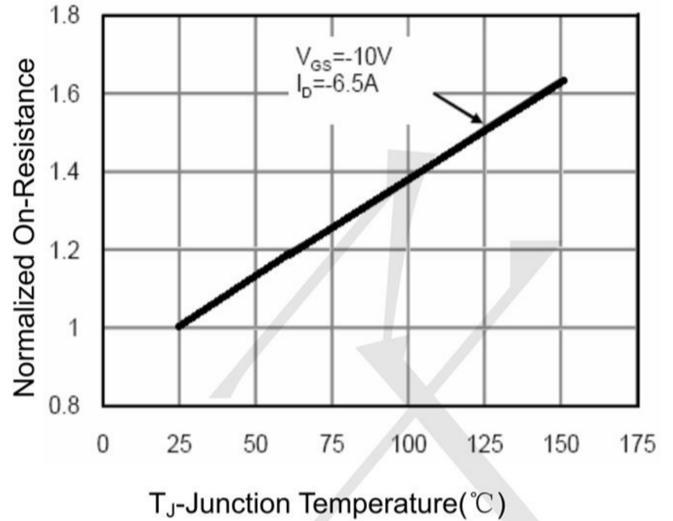
Figure 4 Rdson-Junction Temperature
