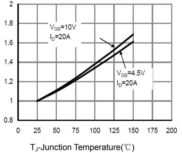
Figure 4 Rds(on)-Junction Temperature
