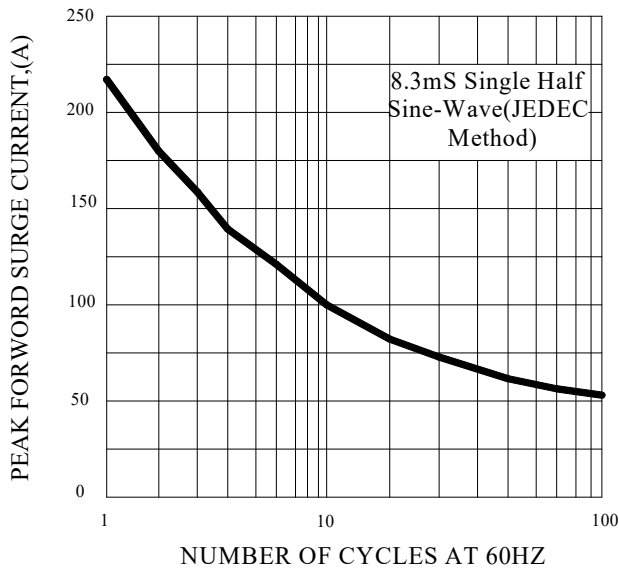
FIG.3-MAXIMUN NON-REPEITIVE FORWARD SURGE CURRENT
