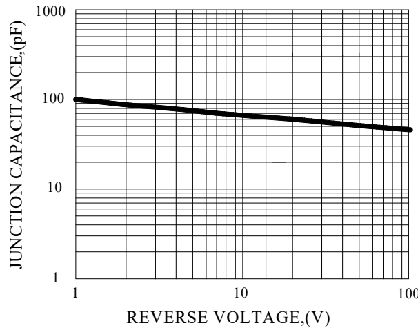
FIG.5-TYPIAL JUNCTION CAPACITANCE
