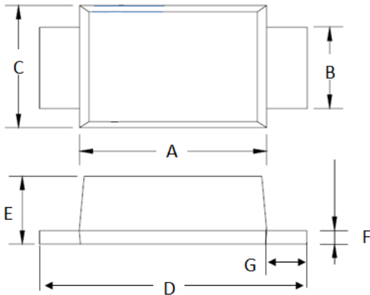
SOD123-F
