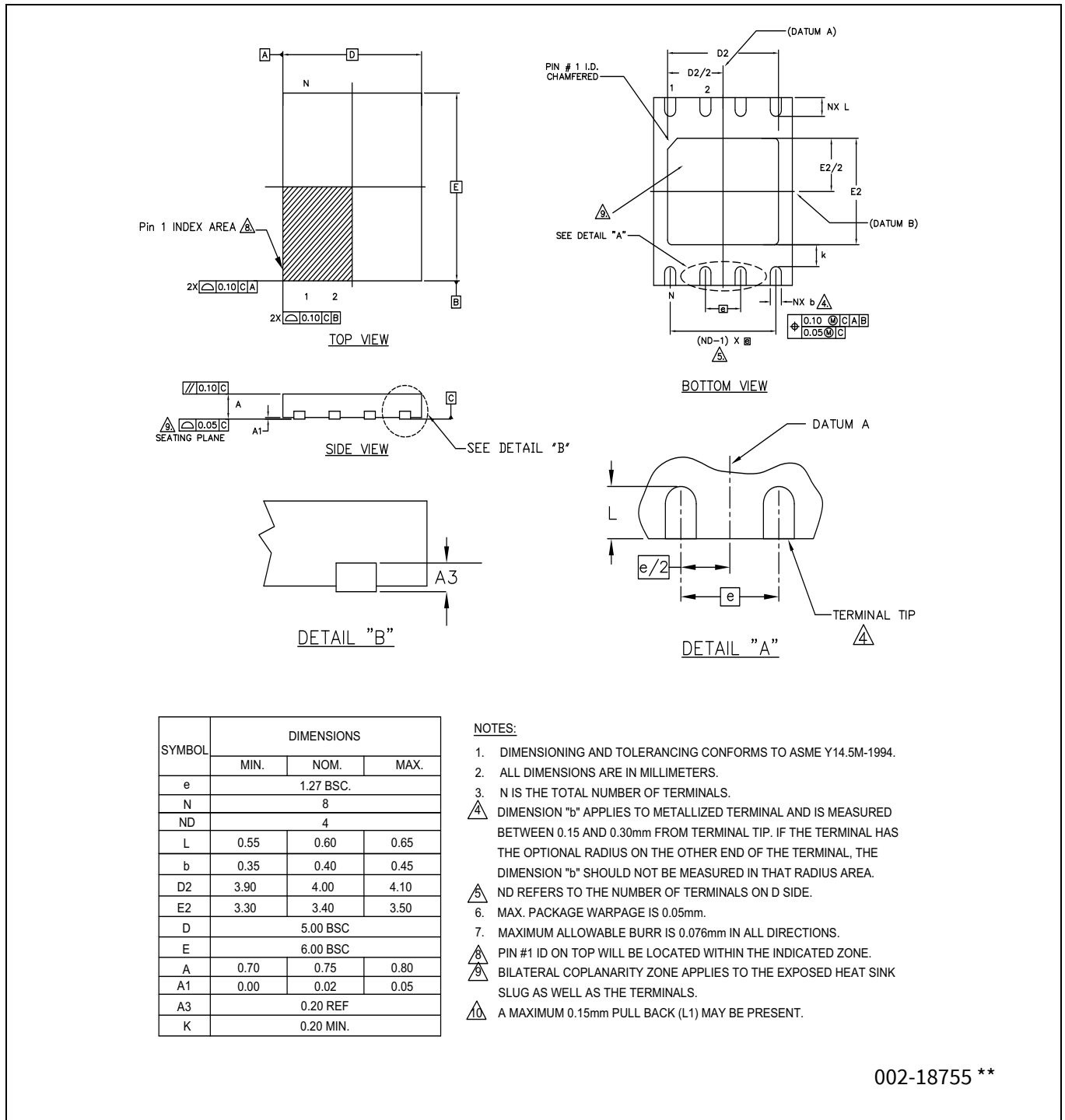
Figure 152 WSON 8-contact 5 x 6 mm leadless (WND008)
