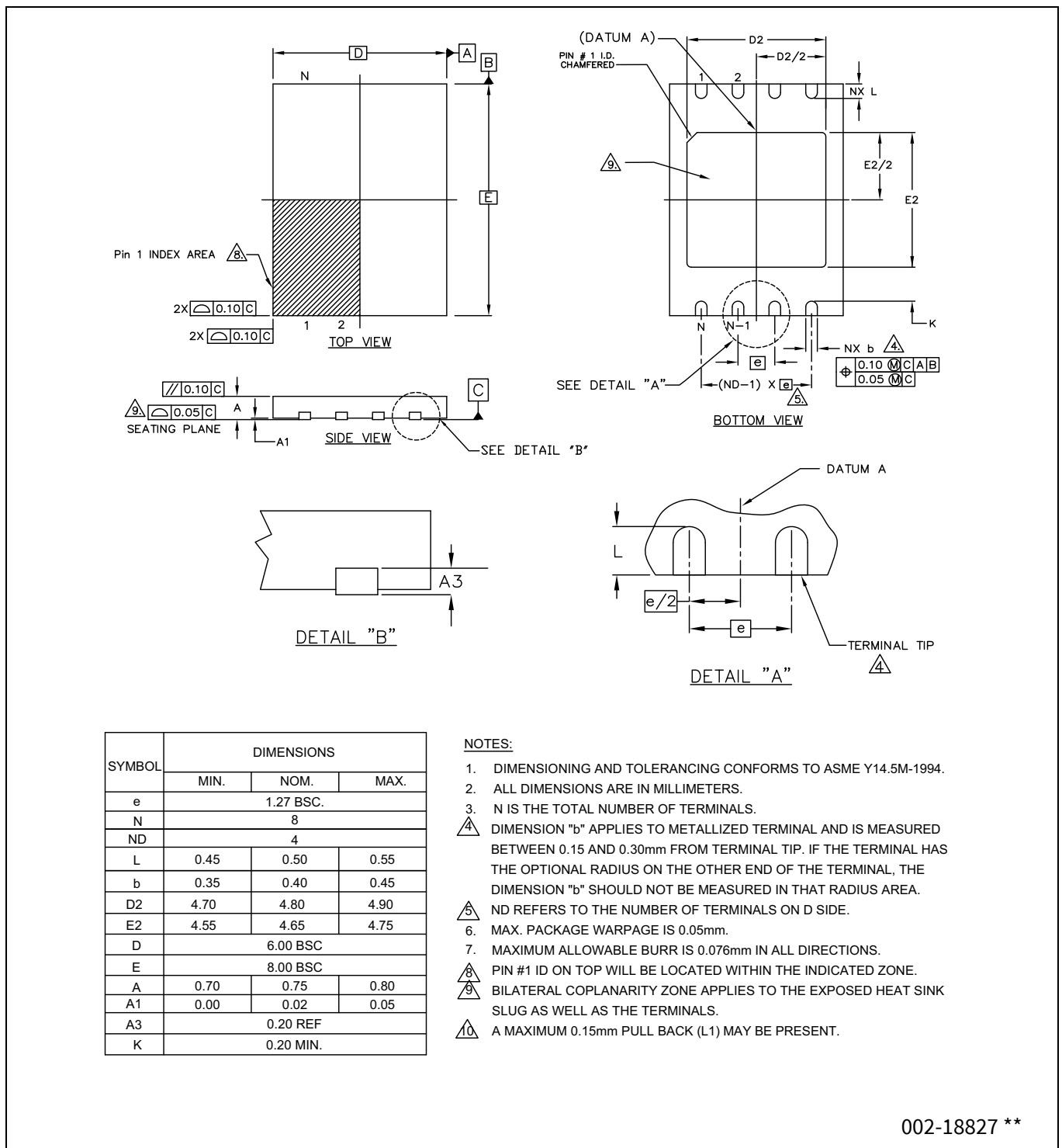
Figure 153 WSON 8-contact 6 x 8 mm leadless (WNG008)
