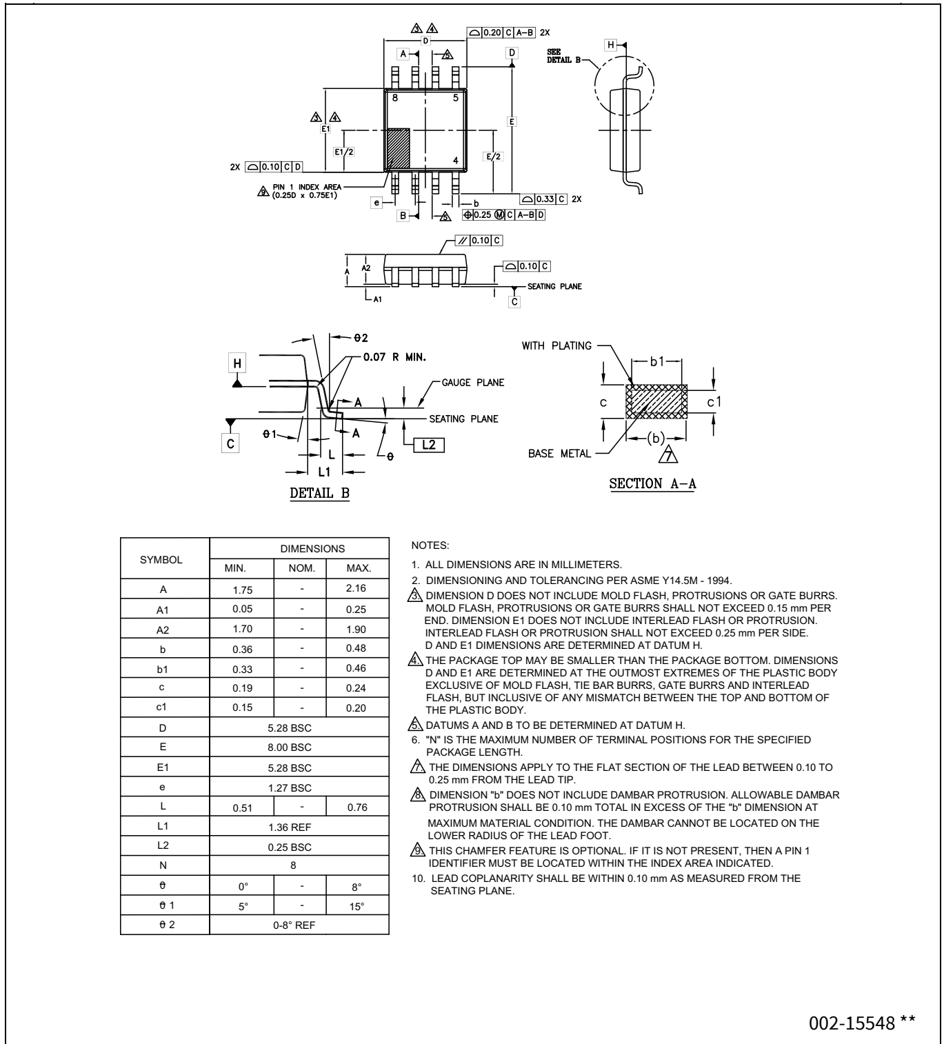
Figure 151 SOIC 8-lead, 208 mil body width (SOC008)
