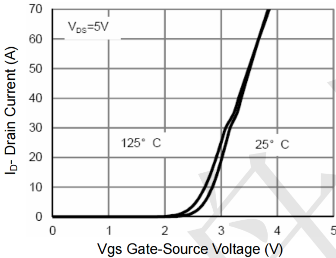
Figure 2 Transfer Characteristics
