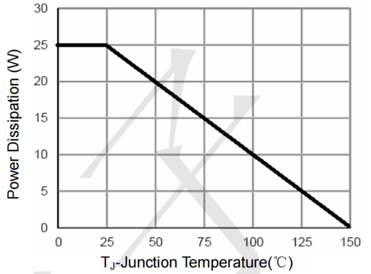
Figure 9 Power De-rating
