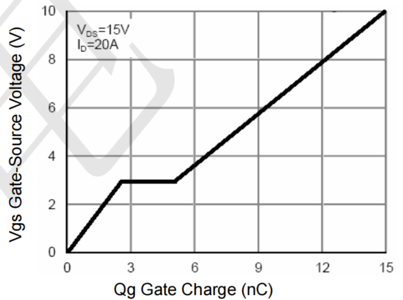
Figure 5 Gate Charge
