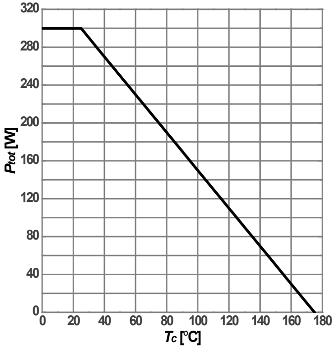
Diagram 1: Power dissipation
