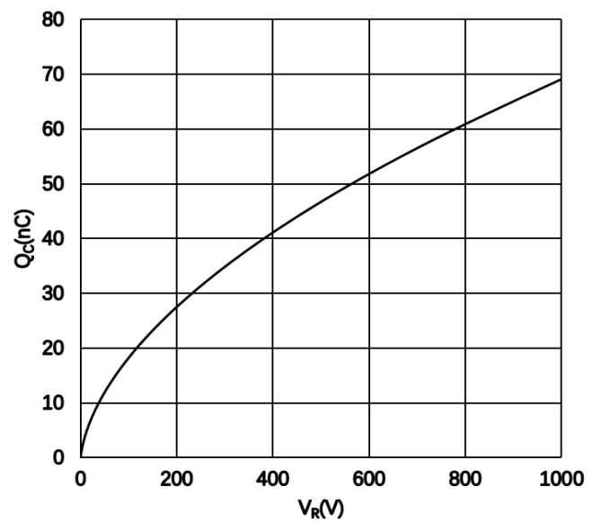
Figure 4. Recovery Charge vs. Reverse Voltage
