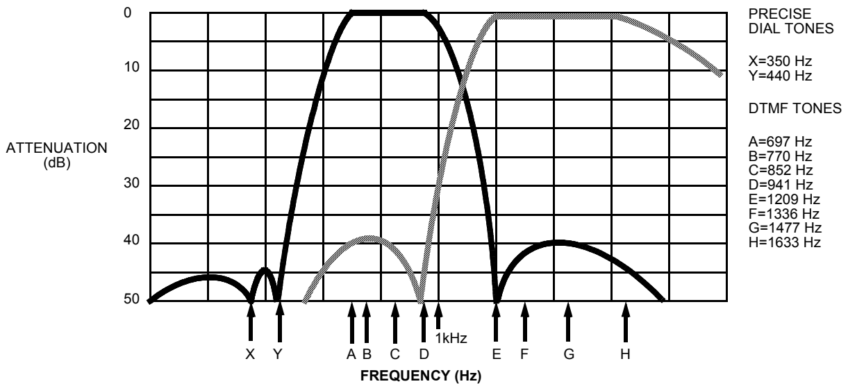
Figure 3 - Filter Response
