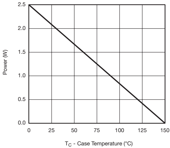
T C - Case Temperature (°C) Power Derating, Junction-to-Foot
