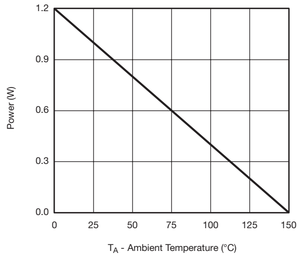
T A - Ambient Temperature (°C) Power Derating, Junction-to-Ambient
