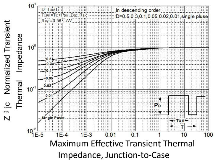
Figure 4: Thermal Transient Impedance
