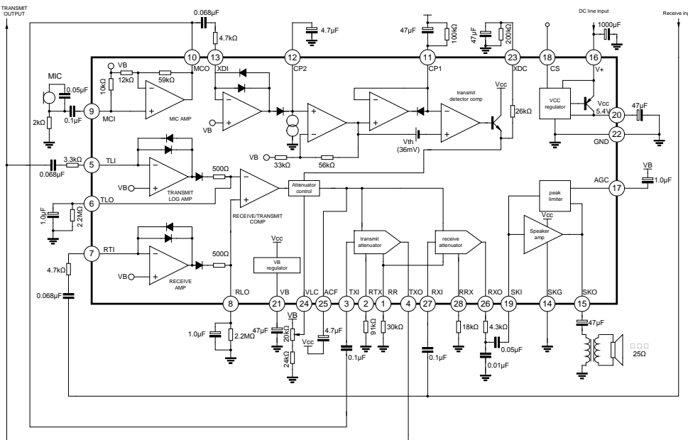
Fig 1 Test circuit
