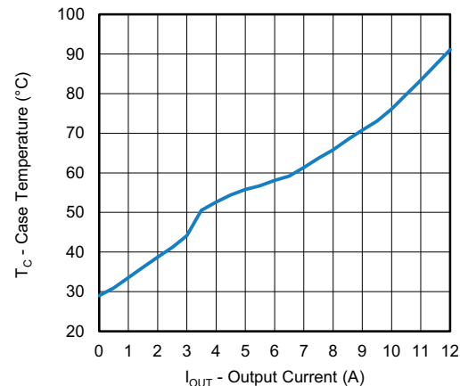
Fig. 15 - SiC476 Load Current vs. Case Temperature, V_{IN} = 48\text{ V} , V_{OUT} = 12\text{ V}
