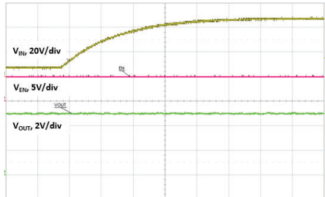
Fig. 50 - Line Transient (8 V to 48 V), Time = 10 ms/div
