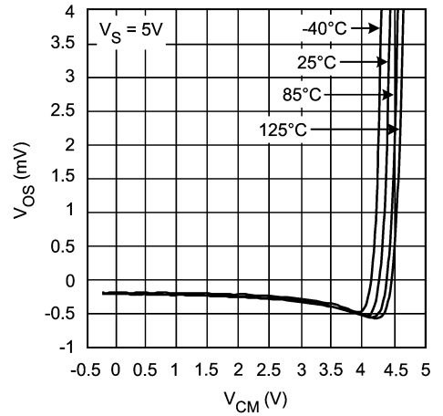
V_{OS} vs. V_{CM} Over Temperature
